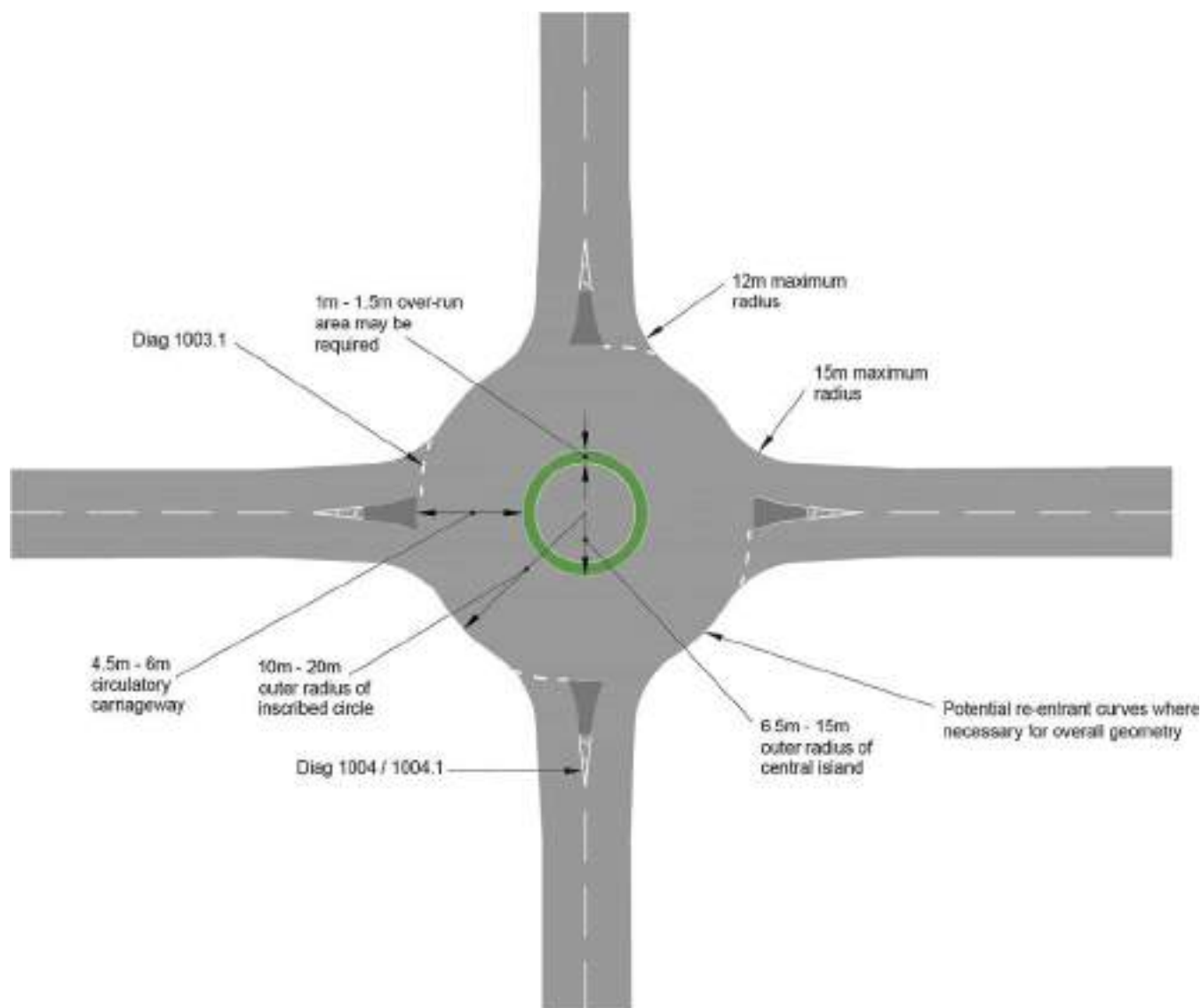
Figure 10.45: Compact roundabout geometry
