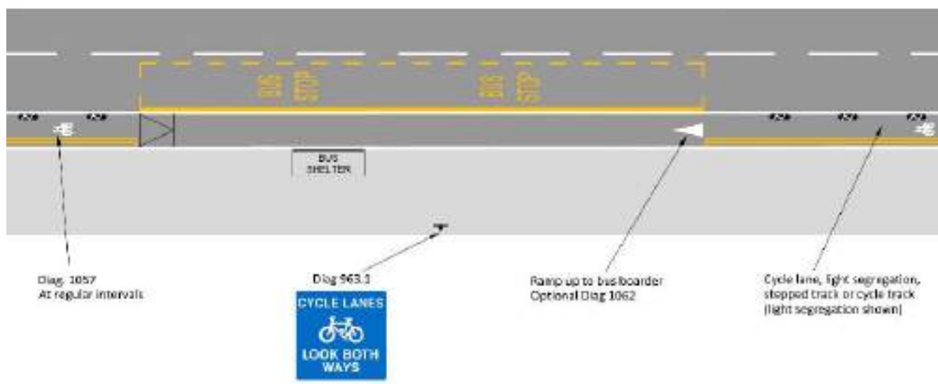
Figure 6.32: Bus stop boarder layout
