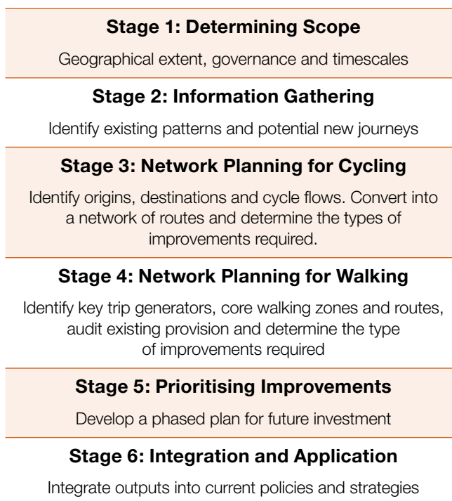
Figure 3.1 LCWIP stages
