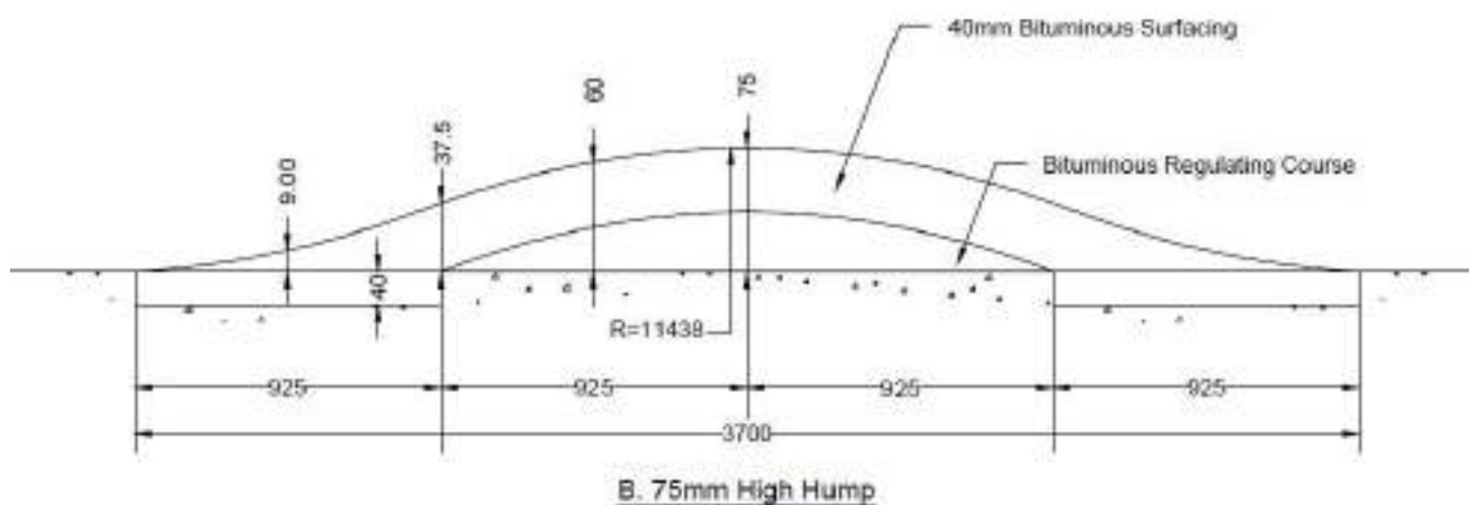
Figure 7.8: Sinusoidal Ramps (Hump may be round or flat-top)
