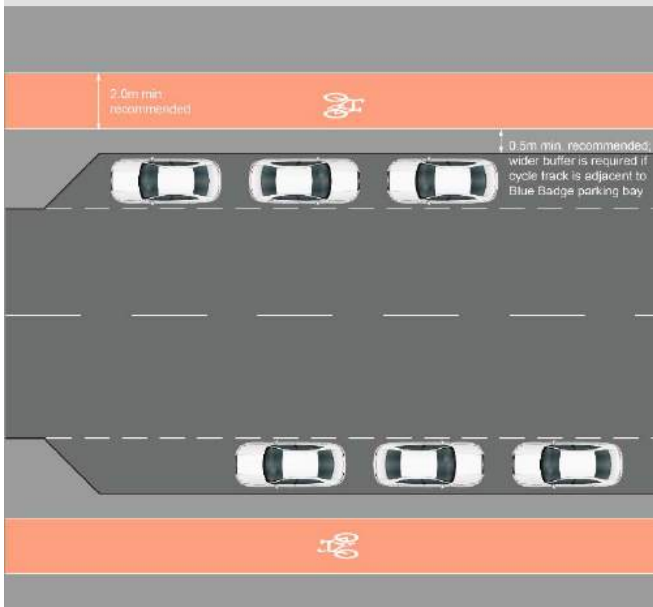
Figure 6.15: Inset parking bays alongside one way cycle tracks
